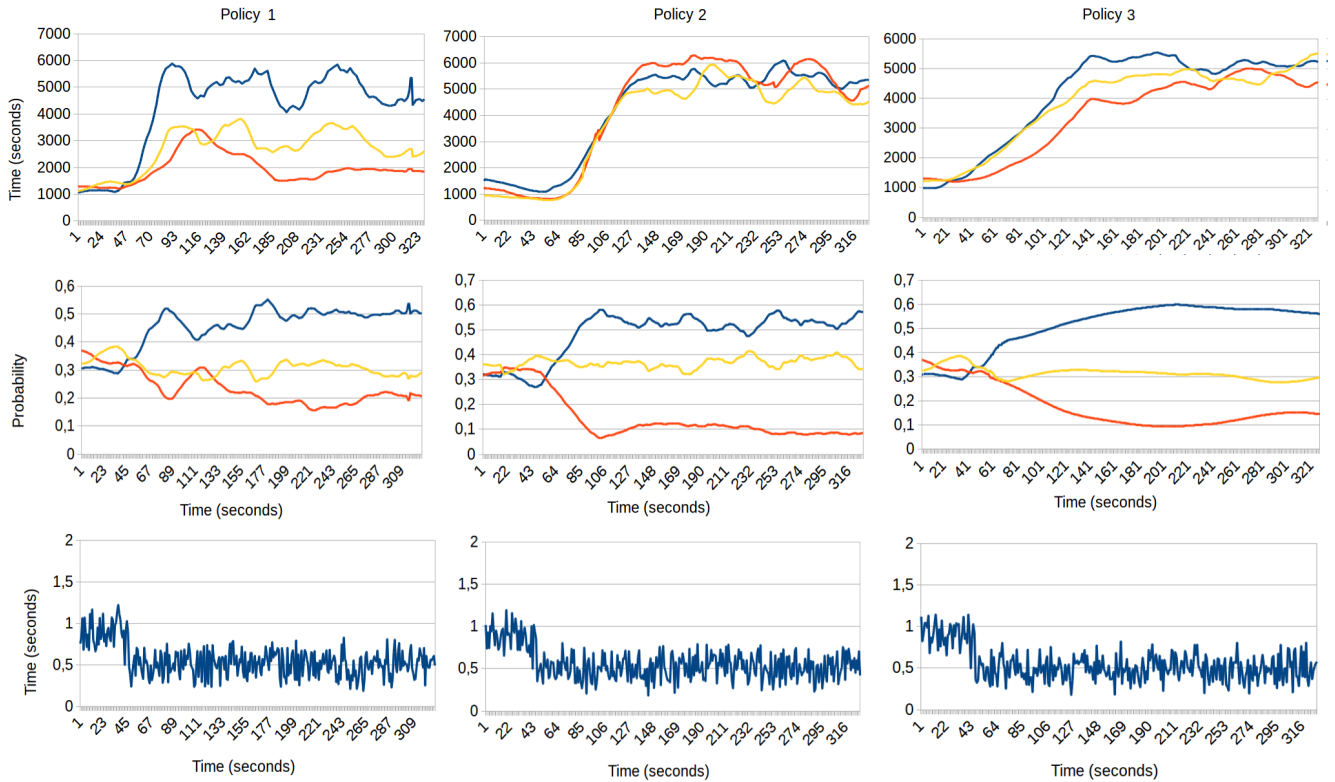
FIGURE 6 Results using 3 regions. The first row shows RMTTF, the second row shows the workload factor f_i , the third row shows the response time measured by the clients of the system.
