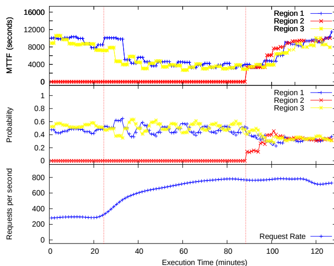
(c) Request rate, MTTF, Forward Probability (3 regions, var. rate)
