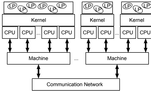
Figure 2.3: Parallel Discrete Event Simulator Multithread Architecture
