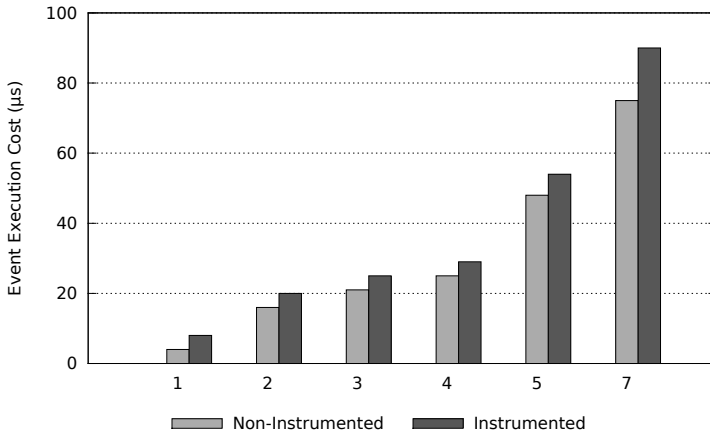
Figure A.4: Overheads Associated with Different Workloads
