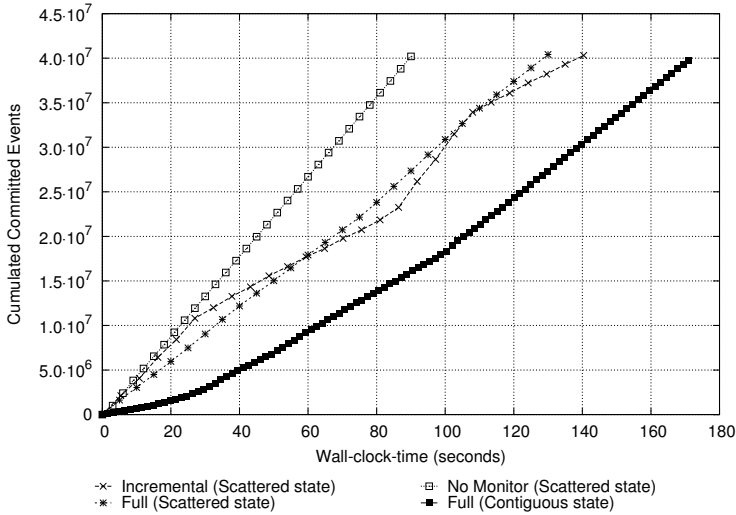
Figure 4.7: PCS – Frequent Fading Recalculation
