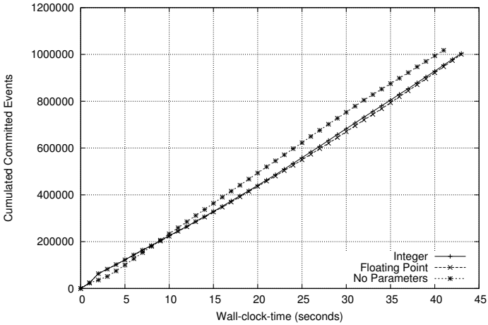
Figure 5.8: Throughput with Different Data Types
