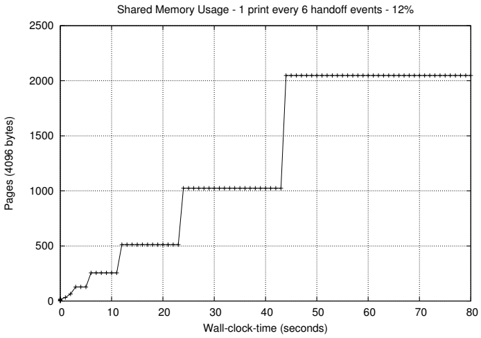
Figure 5.11: Shared Memory Size for f = 12\%
