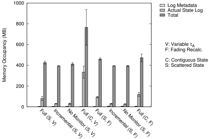
Figure 4.8: PCS – Memory Usage
