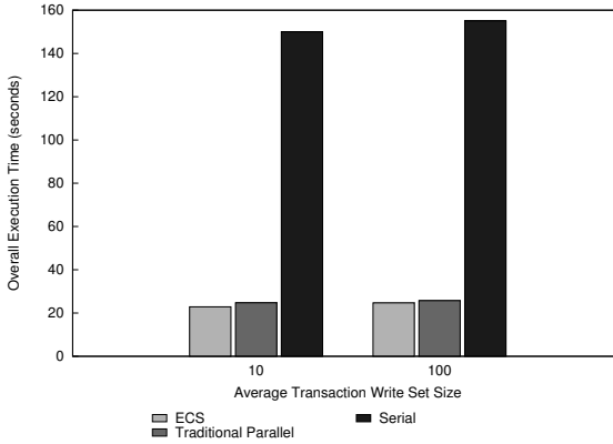
Figure 7.9: Execution times for the NoSQL data store models
