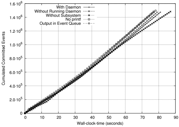
Figure 5.5: Throughput for f = 7\%
