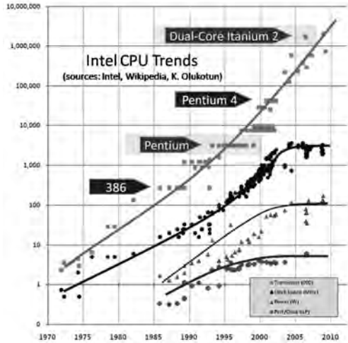
Figure 1.1: CPU specifications trend 1
