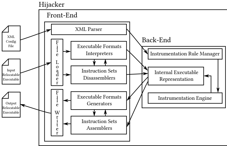
Figure A.1: General Hijacker’s Architecture
