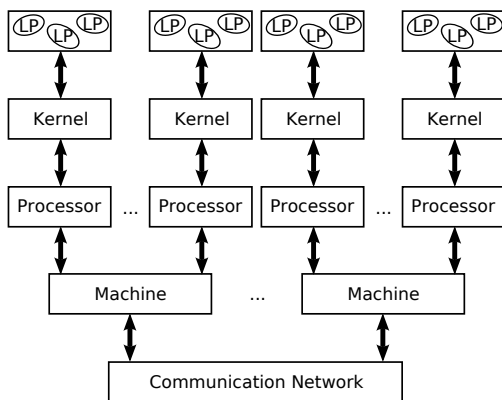
Figure 2.2: Parallel Discrete Event Simulator Classical Architecture
