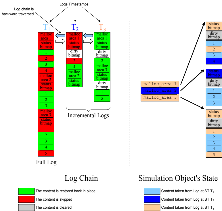
Figure 4.5: Incremental Restore Process
