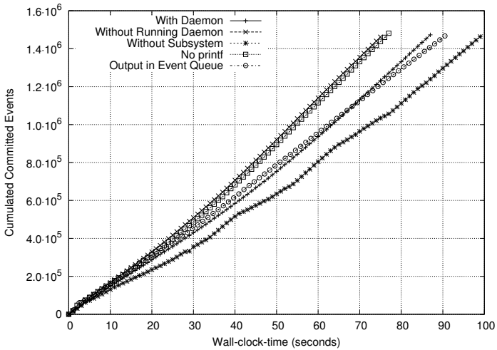
Figure 5.6: Throughput for f = 12\%
