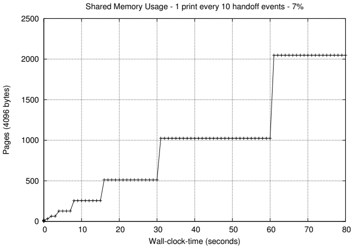
Figure 5.10: Shared Memory Size for f = 7\%
