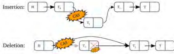
Figure 6.2: Non-Blocking Linked List Operations
