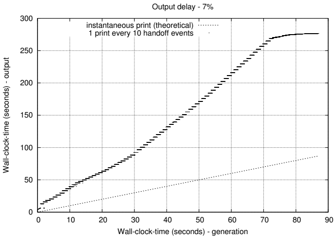
Figure 5.14: Generation/Materialization Delay for f = 7\%
