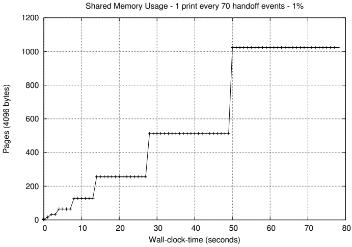
Figure 5.9: Shared Memory Size for f = 1\%
