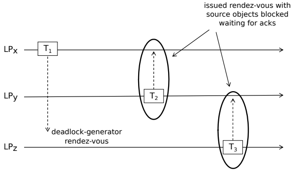
Figure 7.5: Deadlock Originated by a Rendez-Vous Generating Event
