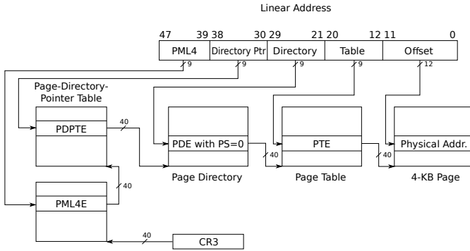
Figure 7.1: The Paging Scheme in x86_64 processors
