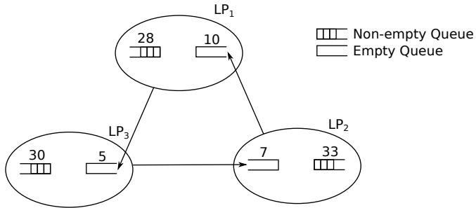
Figure 2.5: Deadlock in Conservative Synchronization
