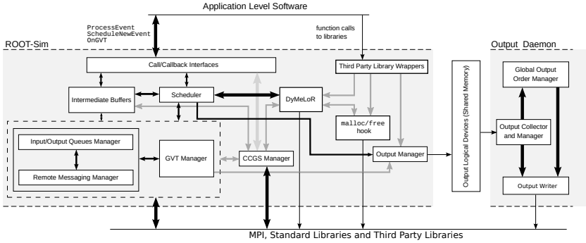
Figure 5.3: ROOT-Sim and the Output Daemon Architecture
