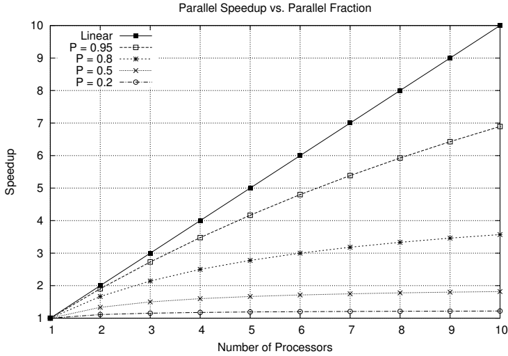
Figure 1.3: Amdahl's Law
