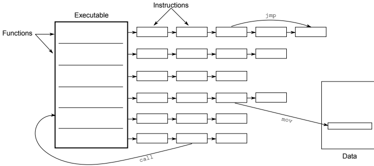
Figure A.3: Hijacker's Internal Representation of Executables
