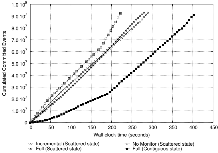
Figure 4.6: PCS – Variable \tau_A
