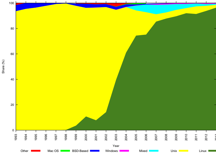
Figure 2.10: Top500: OS share over time
