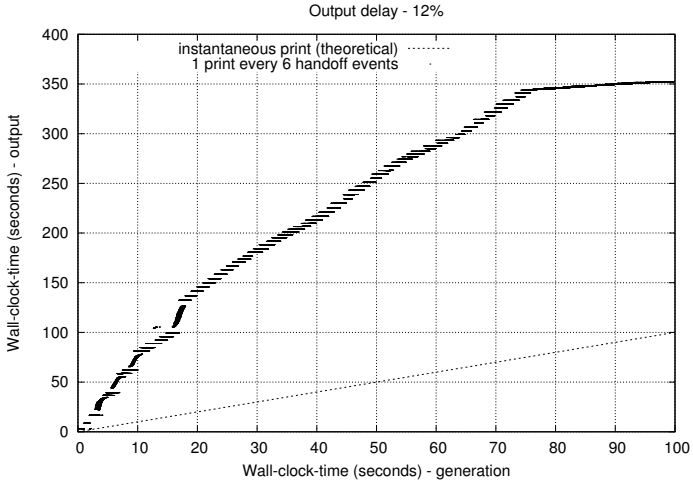
Figure 5.15: Generation/Materialization Delay for f = 12\%
