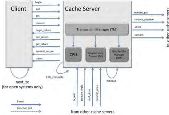
Figure 2.12: Client and Cache-Server LP
