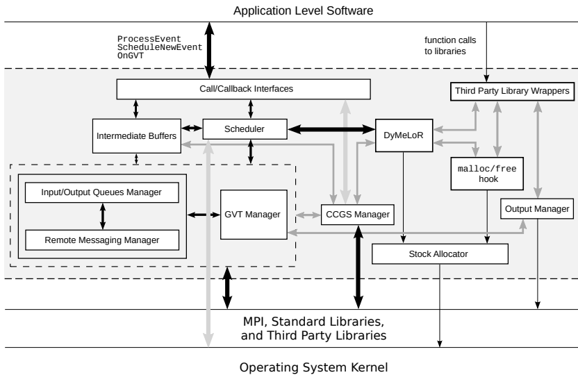
Figure B.1: ROOT-Sim Architecture
