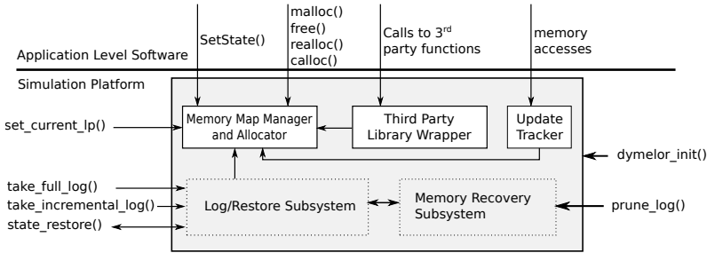
Figure 4.1: Di-DyMeLoR’s Architecture
