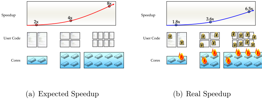
Figure 1.2: Parallel Speedup
