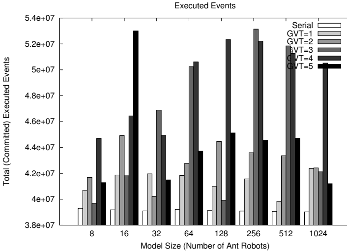
Figure 8.2: Committed Events
