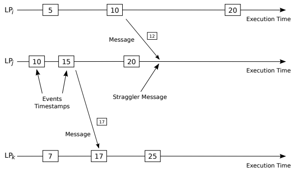
Figure 2.4: Event Causality Violation
