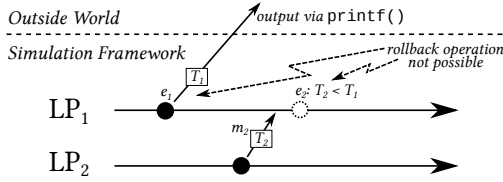
Figure 5.1: Non-Rollbackable Interaction with the Outside World
