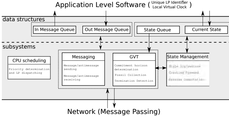
Figure 2.7: Reference Architecture for Optimistic Simulation Systems
