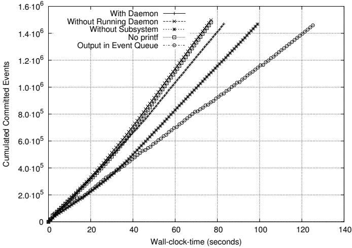
Figure 5.7: Throughput for f = 35\%
