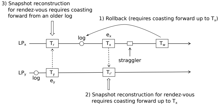
Figure 7.6: Domino-Effect due to a Rollback
