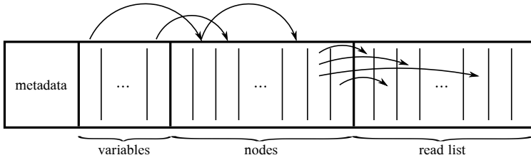
Figure 6.1: Preallocated Shared Memory Map
