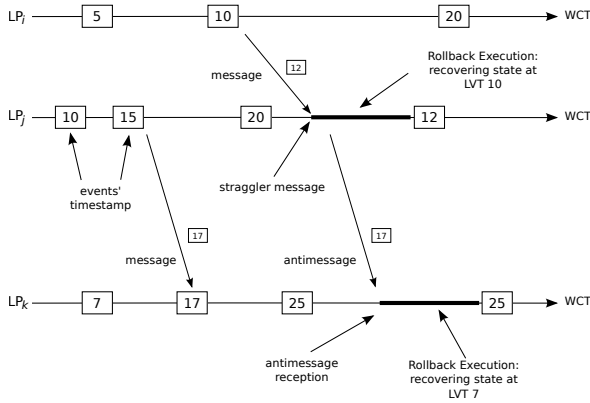
Figure 2.6: Rollback Operation
