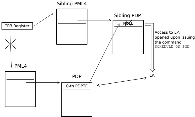
Figure 7.3: LP_x 's Memory Stack is opened for Access
