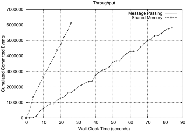
Figure 6.4: Throughput Running on 32 Kernel Instances
