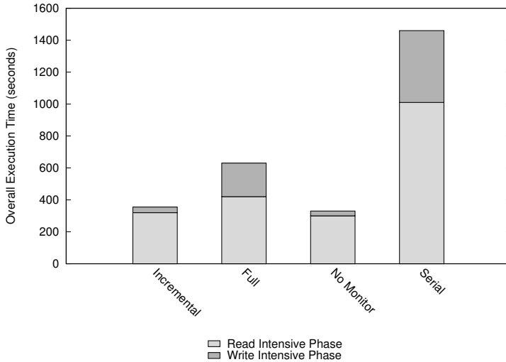
Figure 4.9: NoSQL – Execution Time
